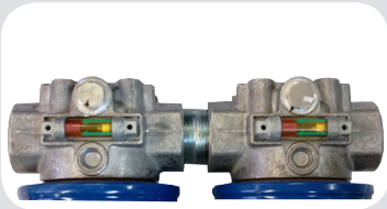
2 x CFLS single heads fitted in series
